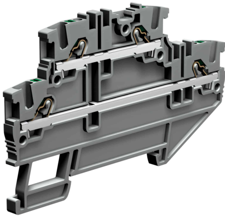
Push-in terminal block 1.5mm 2 , 2-levels, grey color
